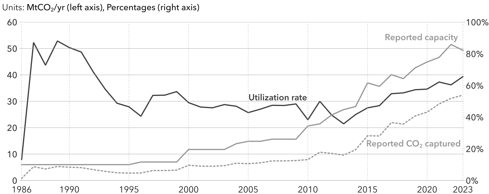
FIGURE 3.2 Reported capacity, reported CO 2 captured, and utilization rates of operational carbon capture projects where available
